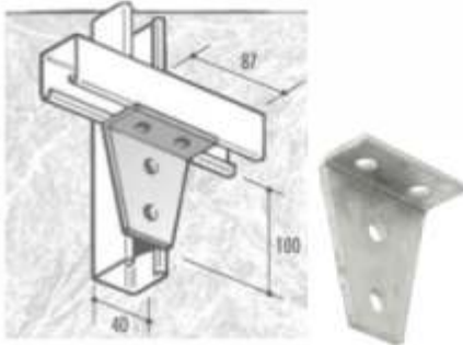
CF-18 90 DEGREE DELTA BRACKET
