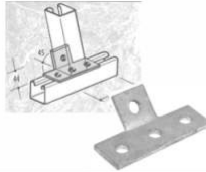
CF-31 ACUTE ANGLED "T" BRACKET
