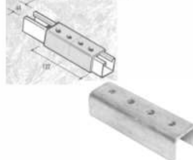
CF-33/41 EXTERNAL CONNECTOR
