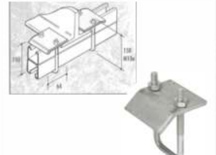
CF-46-UL BEAM CLAMP 'U'BOLT
