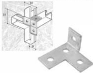
CF-21 90 DEGREE ANGLED RIGHT "T" BRACKET
