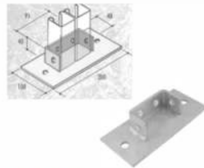
CF-37 BASE PLATE FOR DOUBLE CHANNEL
