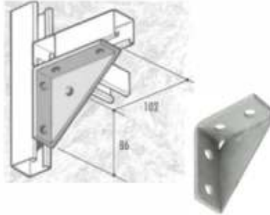
CF-15 SHELF BRACKET
