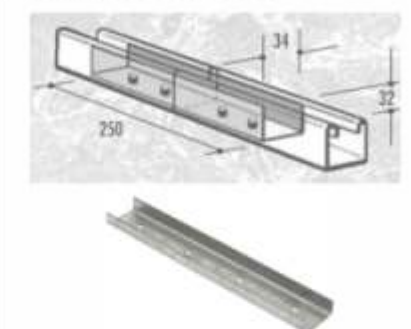
CF-36/21 INTERNAL CONNECTOR
