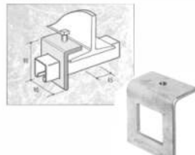
CF-45/41 BEAM CLAMP
