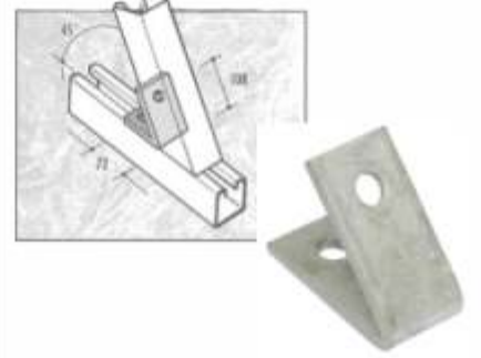
CF-31/45 ACUTE ANGLED "T" BRACKET
