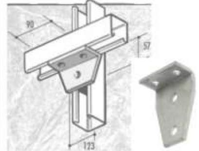
CF-17 90 DEGREE DELTA BRACKET
