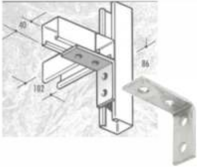
CF-14 90 DEGREE BRACKET
