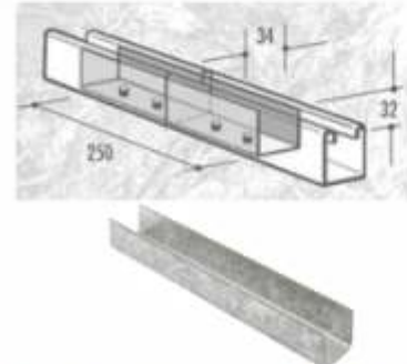
CF-36/41 INTERNAL CONNECTOR
