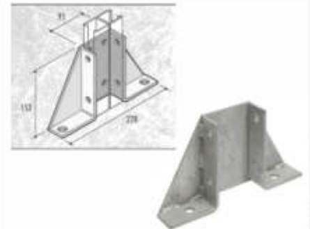
CF-40/82 DOUBLE DELTA BRACKET
