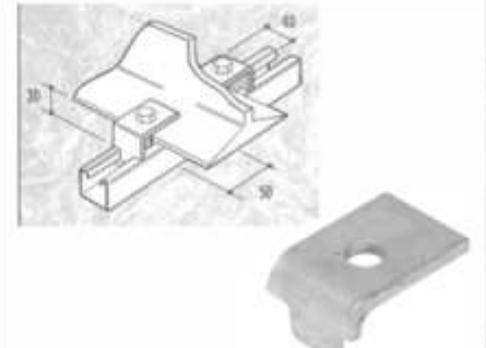
CF-48 BEAM CLAMP
