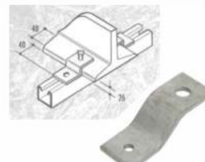
CF-47 'Z' BEAM CLAMP TAPPED M 10
