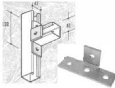
CF-19 90 DEGREE ANGLED "T" BRACKET
