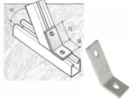
CF-29/45 ANGLED BRACKET
