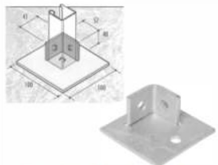
CF-38 BASE PLATE DOUBLE FIX
