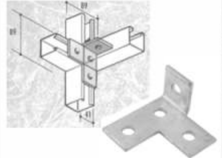
CF-20 90 DEGREE ANGLED LEFT "T" BRACKET
