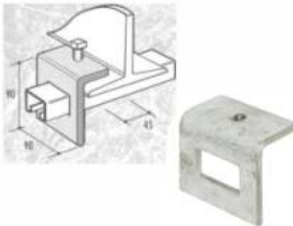
CF-45/21 BEAM CLAMP
