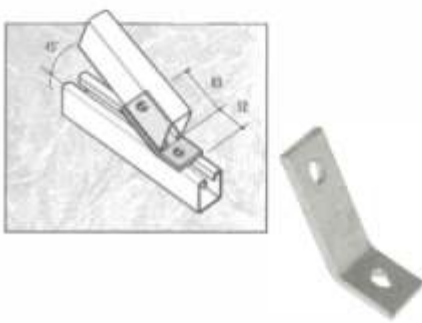
CF-30/45 ANGLED BRACKET
