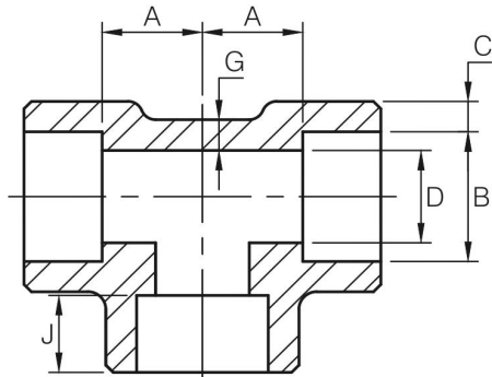
Dimensions are in millimeters.
